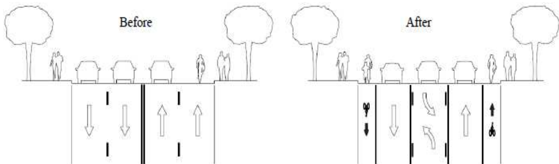
Figure 1: Typical 4 to 3 Reconfiguration.
