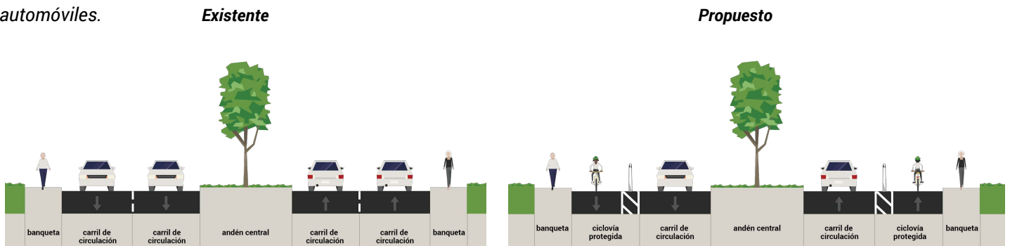
Figura 2 – Corte transversal típica para South Pleasant Valley Road (St. Elmo Road to Onion Creek Park)
