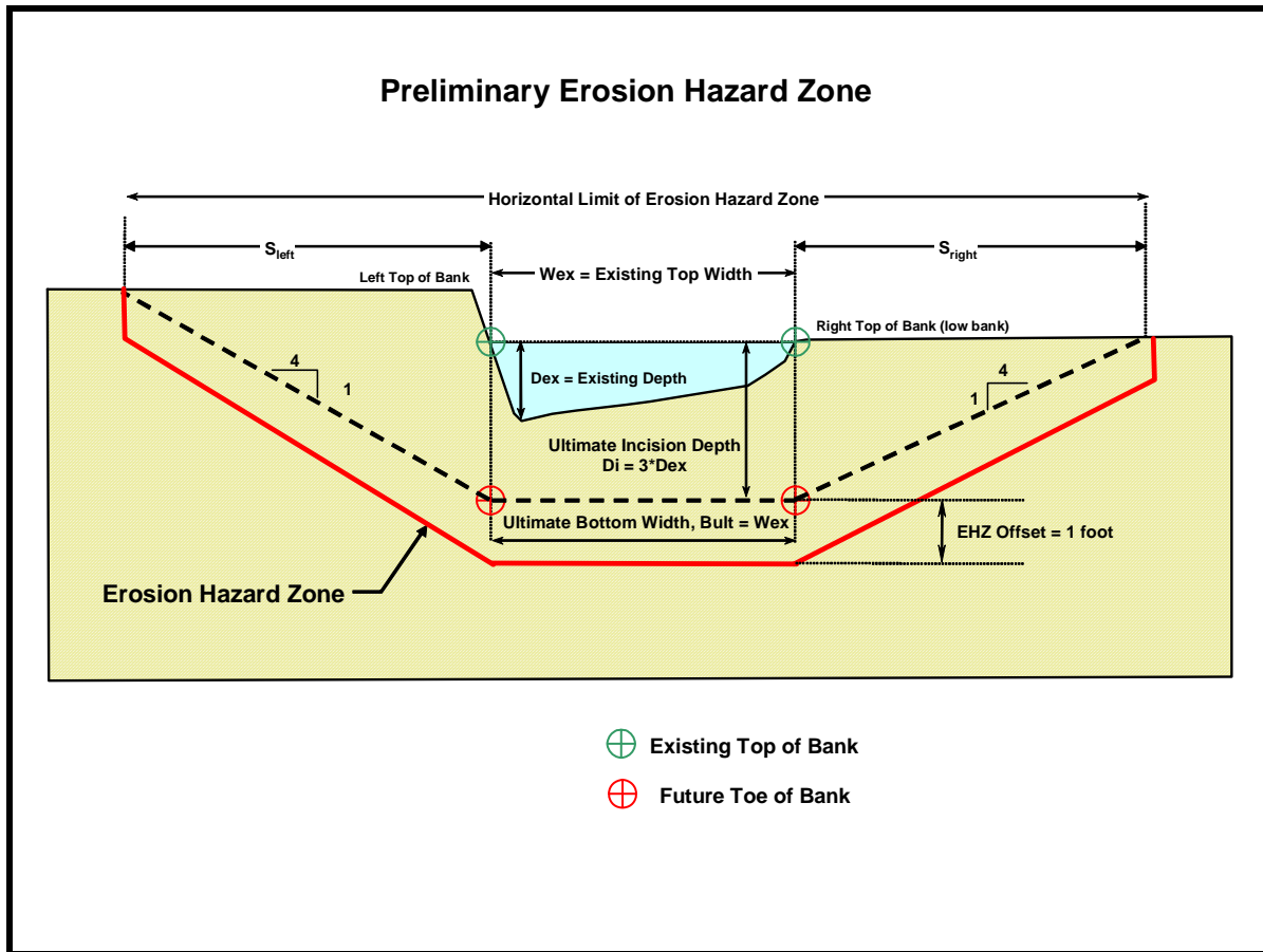
Figure 6. Erosion Hazard Zone Determination
