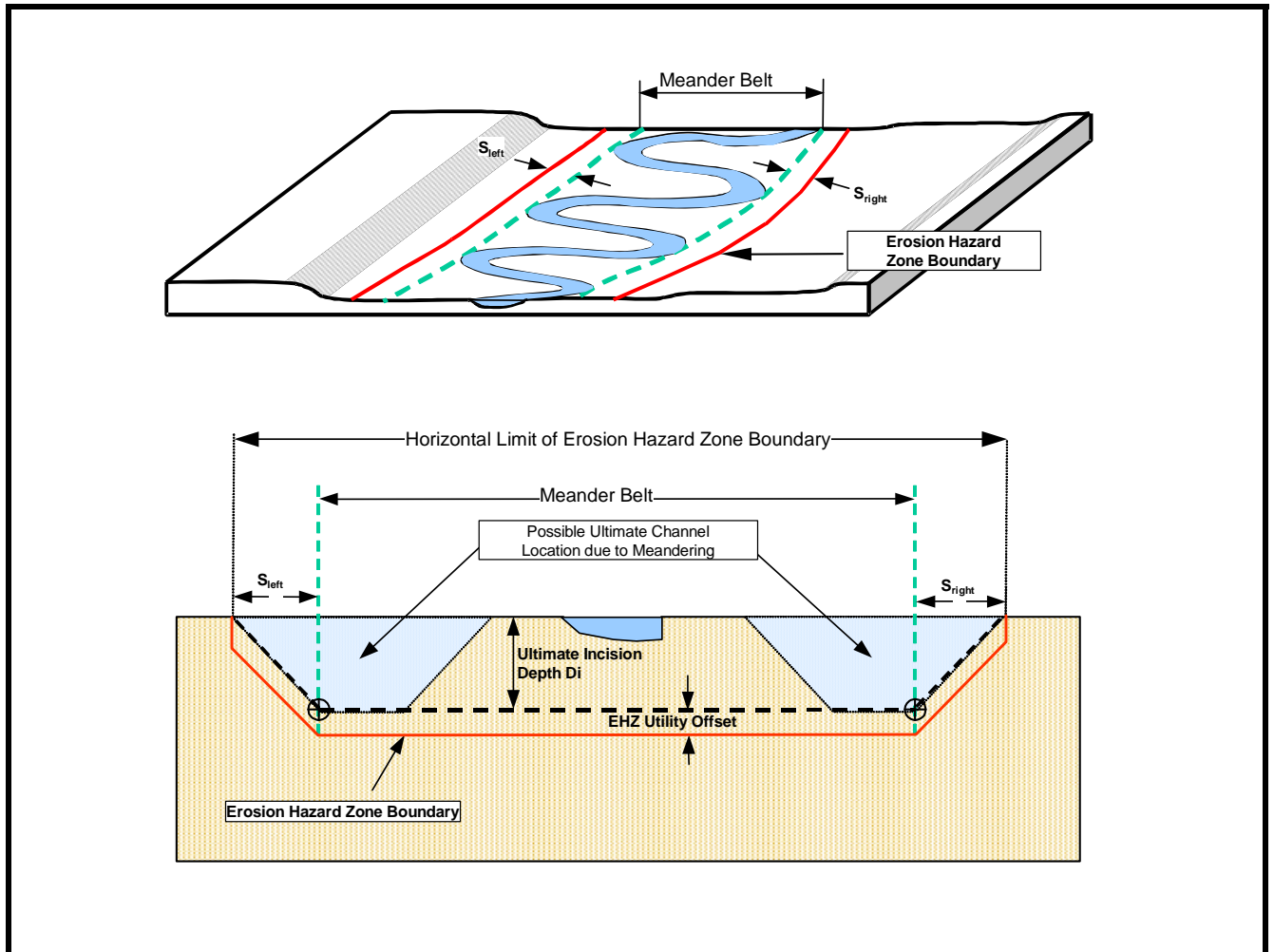
Figure 7. Erosion Hazard Zone Determination for Meandering Streams
