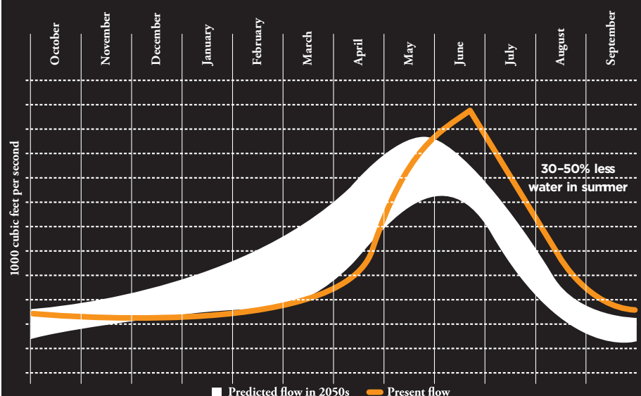
FIGURE 20 PACIFIC NORTHWEST RIVER FLOWS
