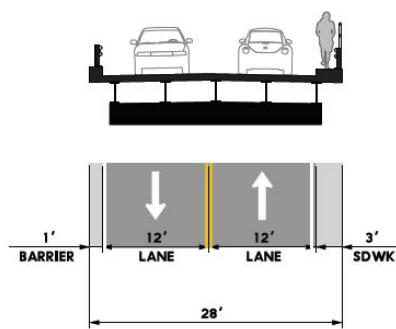
LOOKING EAST EXISTING BRIDGE SECTION
