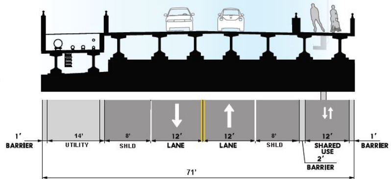
LOOKING EAST PROPOSED BRIDGE SECTION
